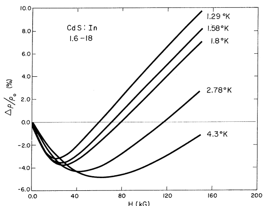
FIG. 3. Magnetoresistance versus magnetic field for sample 1.6-18 at the temperatures indicated ( H \perp I ).
