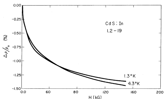
FIG. 4. Magnetoresistance versus magnetic field for sample 1.2-19 at 1.31 and 4.3°K ( H \perp I ).
