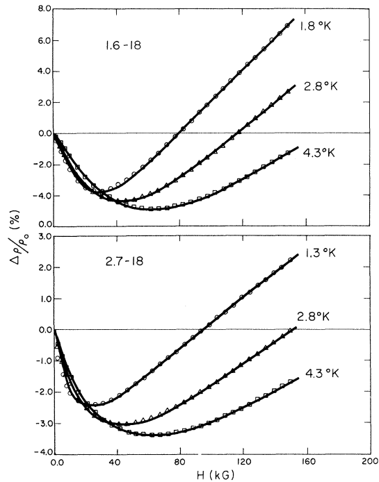
FIG. 9. Representative fits to Eq. (6) of the text for samples 1.6-18 and 2.7-18 at the temperatures indicated.
