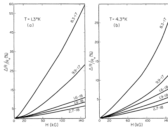
FIG. 11. Relative change in the Hall coefficient \Delta R/R_0 versus H for low-concentration samples 8.3-17 to 2.7-18.
