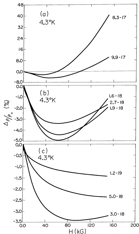
FIG. 5. Magnetoresistance versus magnetic field for various samples at \approx 4.3^\circ\text{K} . Note the change of scales for \Delta\rho/\rho_0 in (a), (b), and (c). A systematic concentration dependence is evident ( H \perp I ).
