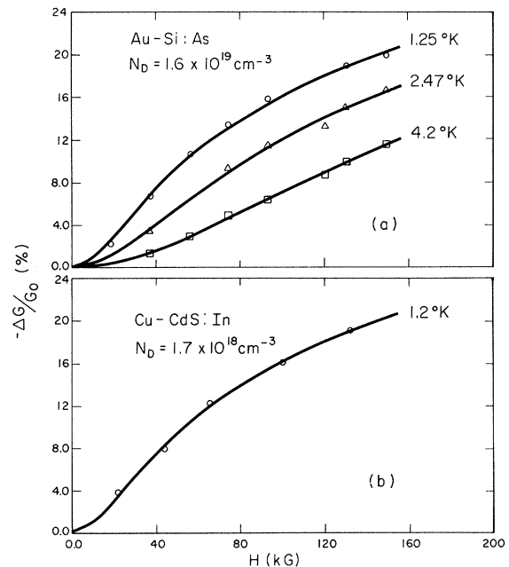
FIG. 19. Tunneling conductance data on Au-Si (Ref. 45) and Cu-CdS (Ref. 43) junctions (analyzed on the basis of the localized-magnetic-moment model by Wolf and Losee) are fitted to our logarithmic empirical expression represented by the solid lines.
