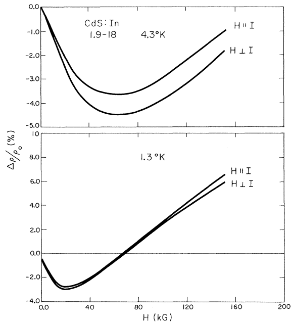
FIG. 10. Comparison of the longitudinal and transverse magnetoresistance for sample 1.9-18 at 4.3 and 1.3 °K.
