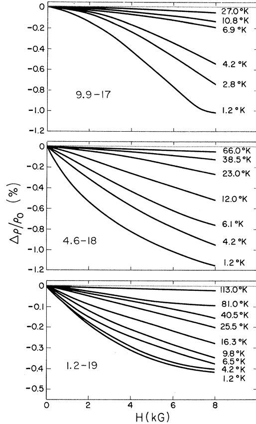
FIG. 2. Low-field magnetoresistance versus magnetic field at various temperatures ( H \perp I ).
