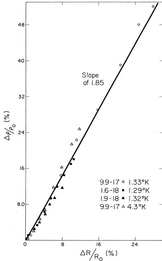
FIG. 17. Plots of derived positive magnetoresistance \Delta\rho/\rho_0 versus relative change in the Hall coefficient \Delta R/R_0 to show that magnetic freeze-out effects are responsible for the positive component. (See Ref. 25.)
