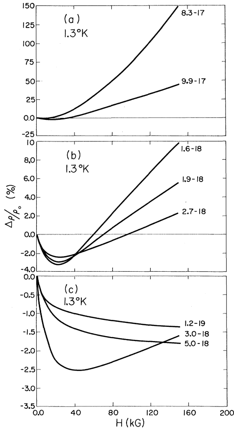
FIG. 6. Magnetoresistance versus magnetic field for various samples at \approx 1.3^\circ\text{K} . Note the change of scales for \Delta\rho/\rho_0 in (a), (b), and (c). A systematic concentration dependence is evident ( H \perp I ).
