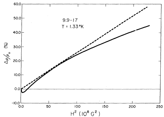
FIG. 12. Magnetoresistance versus H^2 for sample 9.9-17 at 1.33 °K, representative of the fact that, for lower concentration samples, as the magnetic field increases the positive component deviates from the H^2 dependence ( H \perp I ).
