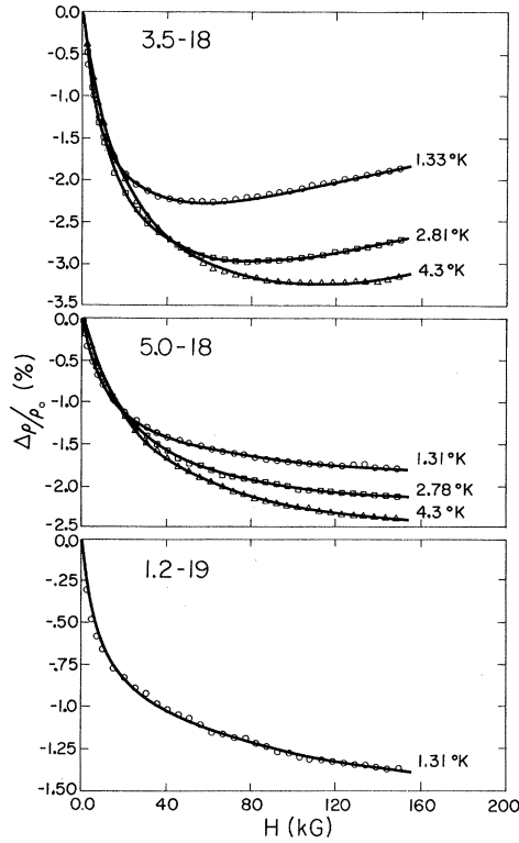
FIG. 14. Least-squares fits to the empirical logarithmic expression (represented by the solid lines). For samples 3.5-18 and 5.0-18 there is an admixture of small positive component [expression (18)]. Sample 1.2-19 is fitted to expression (17) of the text only.
