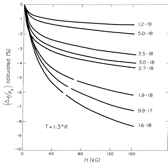
FIG. 16. Calculated negative component of magnetoresistance for various samples using the values of the fitted parameters B_1 and B_2 .
