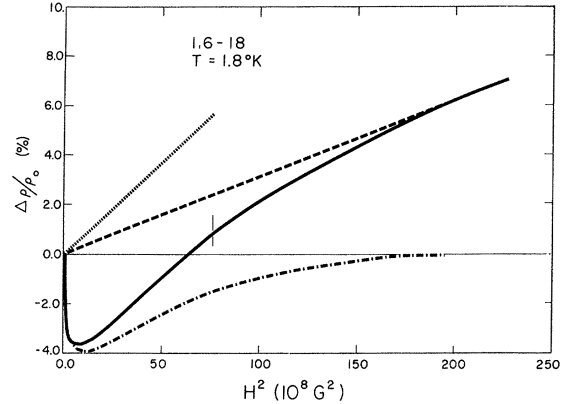
FIG. 8. Magnetoresistance versus H^2 for sample 1.6-18 at 1.8°K. Solid line represents experimental data; dotted line represents conventional positive component if the data were taken only up to \approx 75 kG (indicated by the vertical line); dashed line represents the positive component as a result of the extrapolation of the high-field data to pass through the origin; dot-dashed line represents the negative component obtained by subtracting the observed magnetoresistance from the dashed line.
