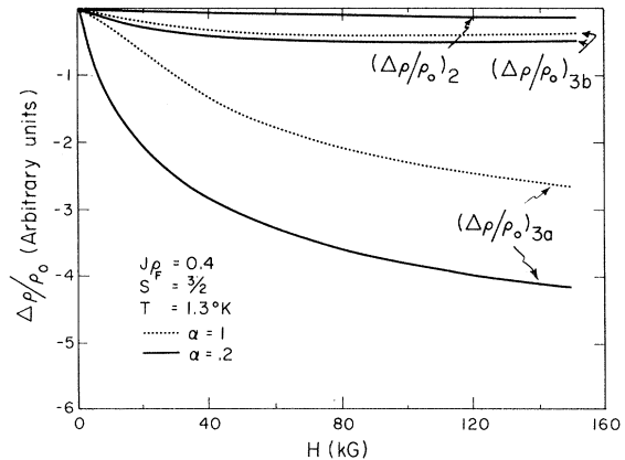
FIG. 18. Calculations of (\Delta\rho/\rho_0)_2 , (\Delta\rho/\rho_0)_{3a} , and (\Delta\rho/\rho_0)_{3b} in expression (13) of the text for the values of the parameters indicated to show that (\Delta\rho/\rho_0)_{3a} is the dominant term.
