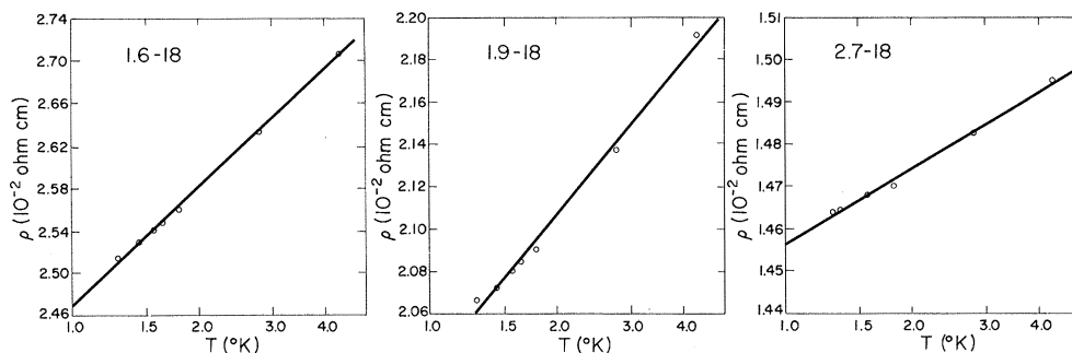
FIG. 13. Resistivity versus log temperature. (Solid lines are the fits to the equation \rho = a + b \ln T .)
