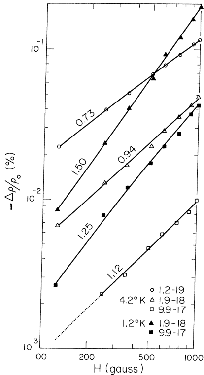
FIG. 7. Negative magnetoresistance versus magnetic field between 125–1000 G to show that \Delta\rho/\rho_0 \propto H^n , where n < 2 ( H \perp I ).
