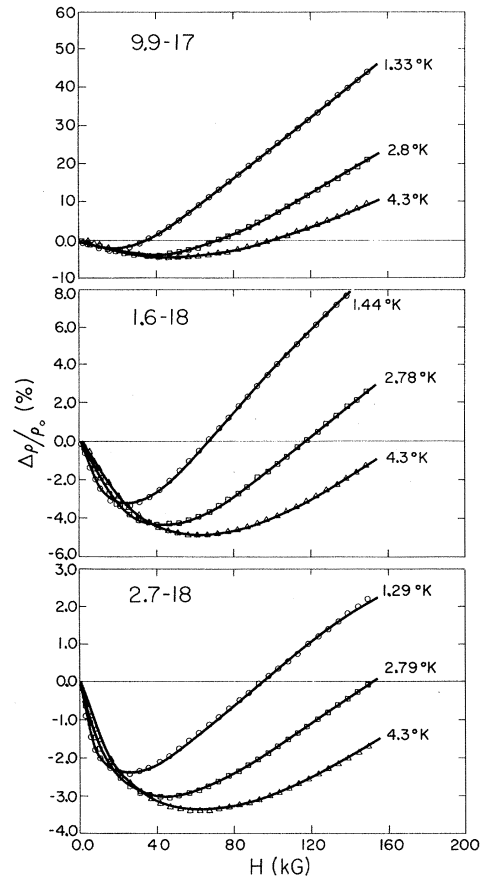
FIG. 15. Least-squares fits to the compound expression (18) (represented by the solid lines) for various samples at the temperatures indicated.
