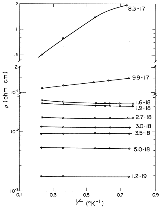
FIG. 1. Resistivity versus 1/T . (Sample numbers represent the room-temperature carrier concentration, e.g., 8.3-17 \equiv 8.3 \times 10^{17} \text{ cm}^{-3} , etc.)
